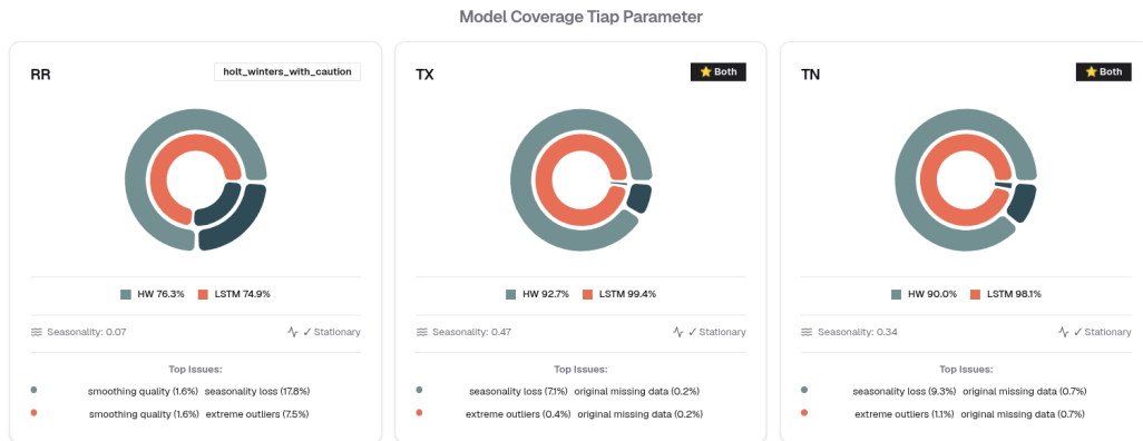
Gambar 4.14. Model Coverage
