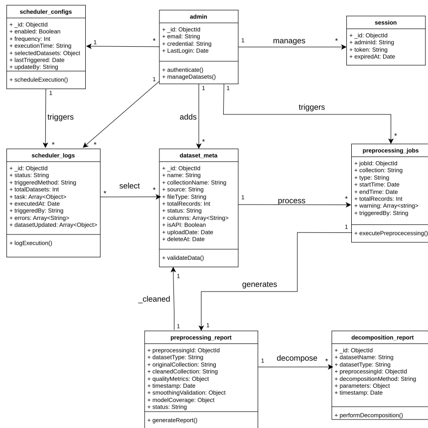
Gambar 4.19. Class Diagram
